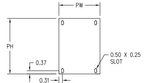
BACK PANEL DIMENSIONS (PANEL INCLUDED)
